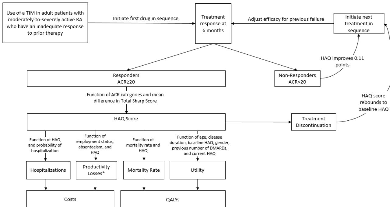
Figure 8. Model Framework
