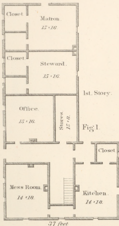
PLAN OF A TWO STORY HOSPITAL.
