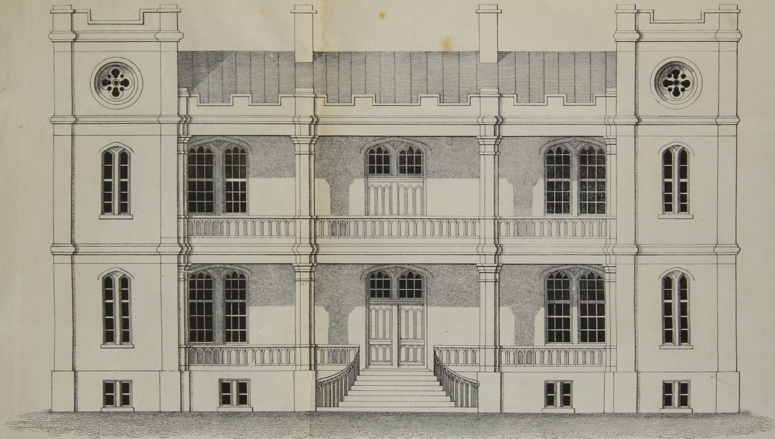
FACADES OF MARINE HOSPITAL TO ACCOMMODATE 50 PATIENTS BESIDES OFFICERS ROOMS & C.
