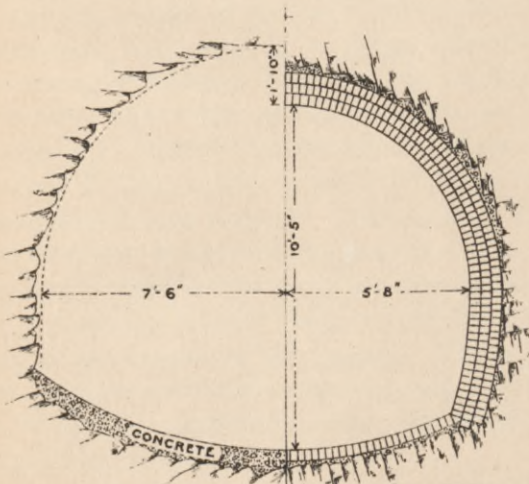
HALF SECTION UNLINED TUNNEL.
