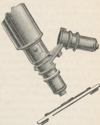
Fig. 42.—BENT NOSE-PIECE.
