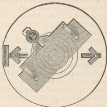
Fig. 67.—COX TURN-TABLE.
