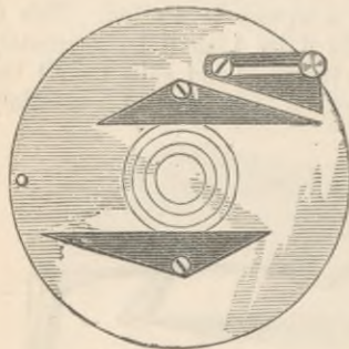
Fig. 63.—MATTHEW'S TURN-TABLE.
