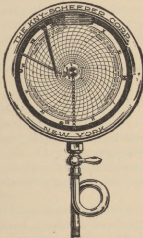
Fig. 17.—Sterilizing-room detector.
