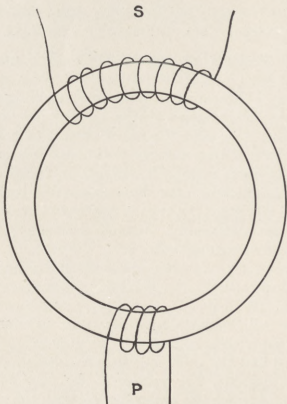
FIG. 15.—Ring type of transformer.
