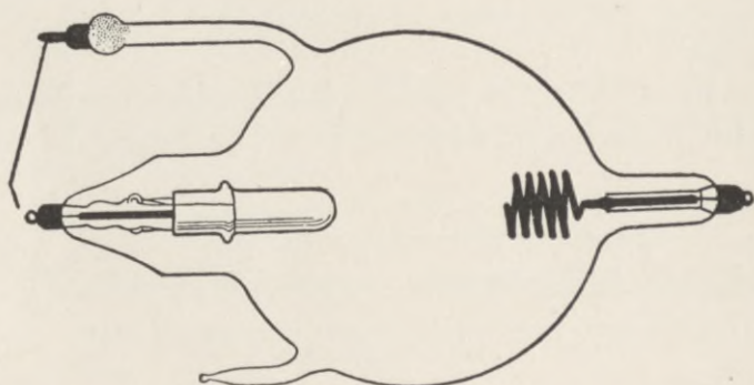
FIG. 12.—Valve tube.
