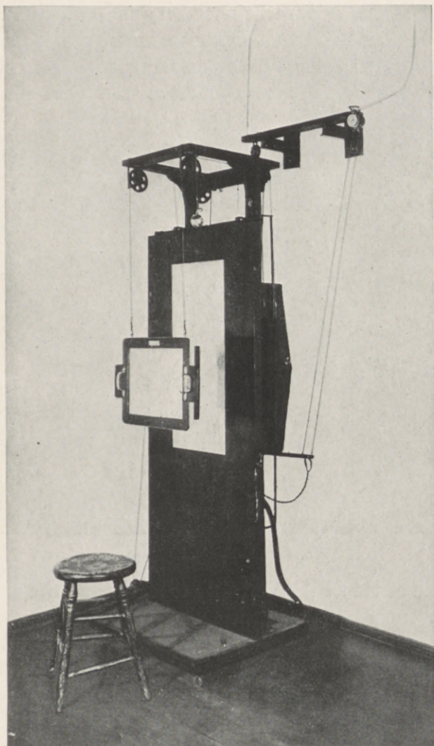
FIG. 22.—The upright roentgenoscope.
