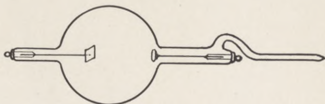
FIG. 6.—Jackson's focus tube.
