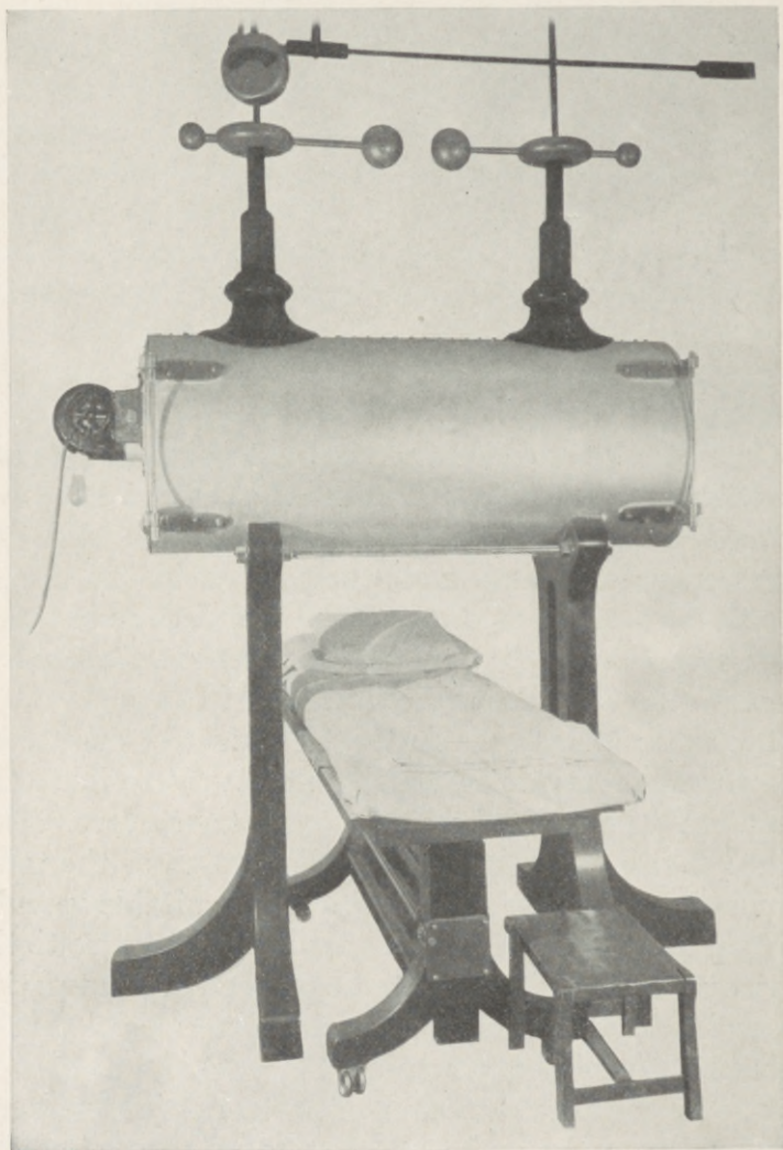
FIG. 177.—Lead cylinder enclosing Coolidge tube designed for voltages of 200,000 and upward. The table is adjustable in height.
