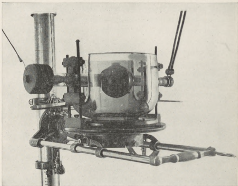
FIG. 10.—Radiator type of Coolidge tube.
