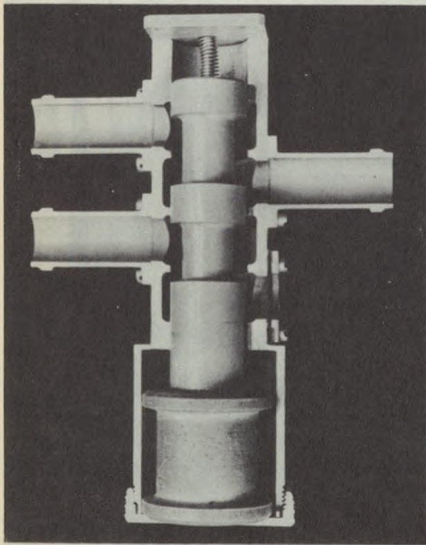
Figure 3-5. —The Standard G-valve, at 1 G. Under this condition pressure from the left normally escapes through an exhaust at the lower right. As G lowers the central column on the spring, part of the pressure escapes via the upper right tube to the suit. After G is removed, this suit pressure then escapes via the small opening at the upper left which was closed during G.
