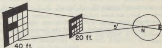
Figure 4-3.—Each letter subtends a 5' angle at the nodal point (N). Each point of separation of the letter subtends a 1' angle.
