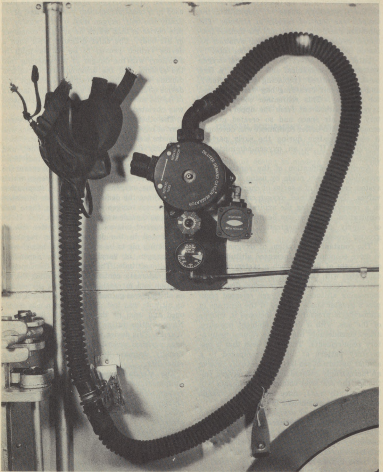
Figure 2-5.—Diluter-demand regulator, oxygen flow indicator and pressure gauge, with type 14 mask attached to quick release disconnect.
