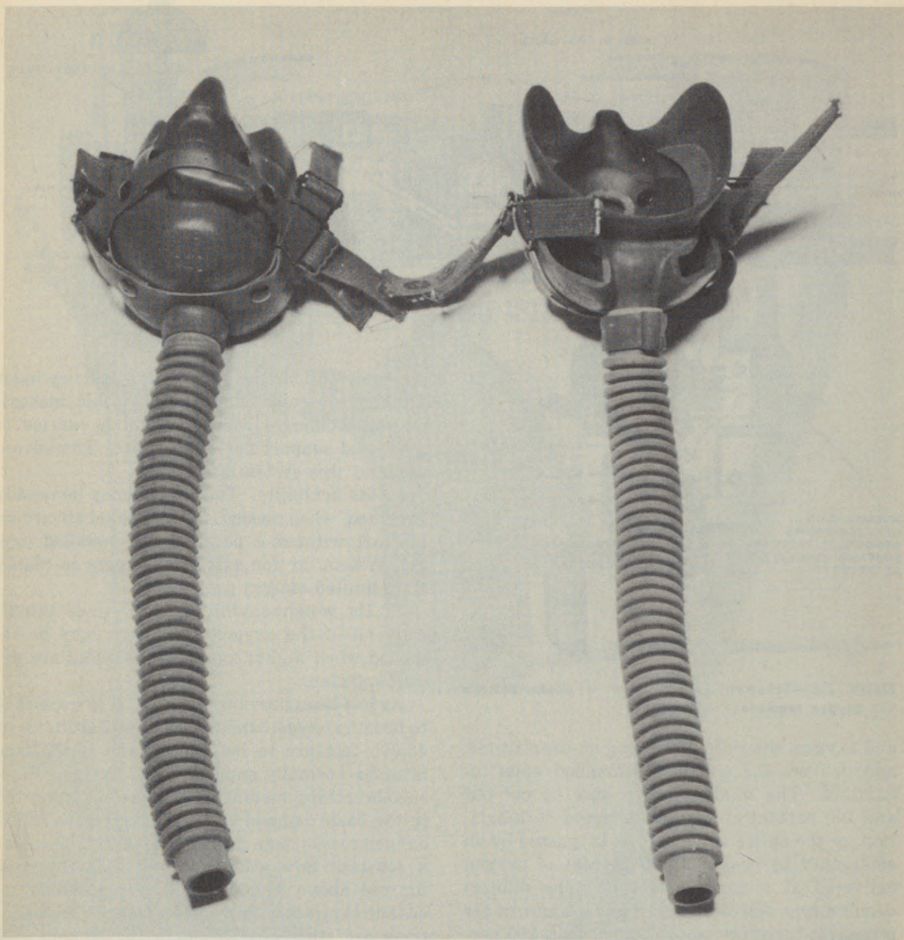
Figure 2-7.—Type 14 oxygen mask for use with standard diluter-demand aviator's oxygen equipment.
