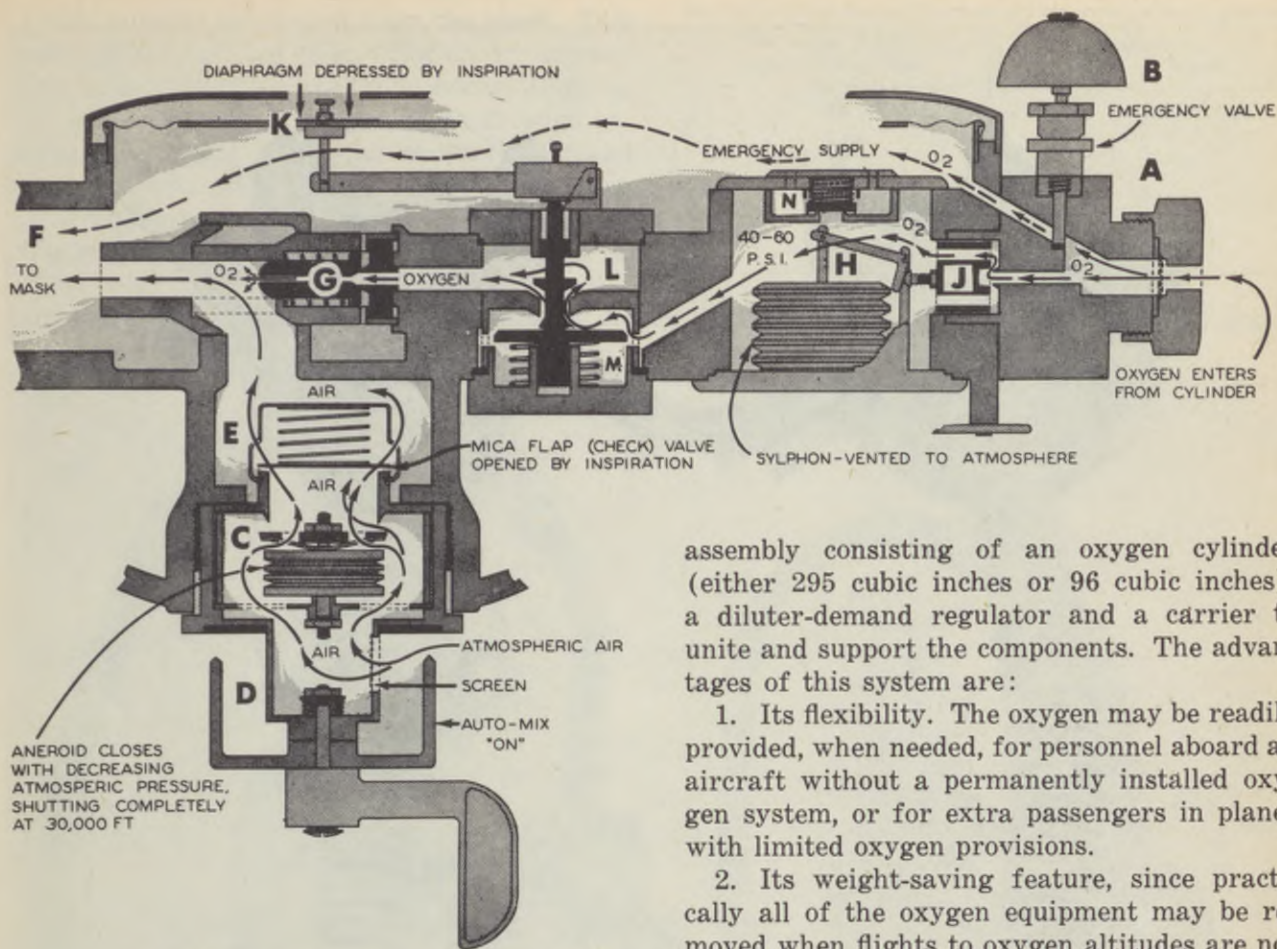
Figure 2-6.—Schematic diagram of a diluter-demand oxygen regulator.
