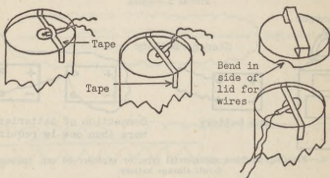
FIGURE 4.—Method of attaching squib.
