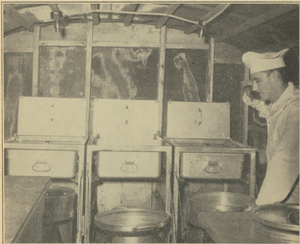
Plate 26. Illustrating the arrangement of the field ranges, the lighting setup and the slats fastened across the bows to support the screening.
