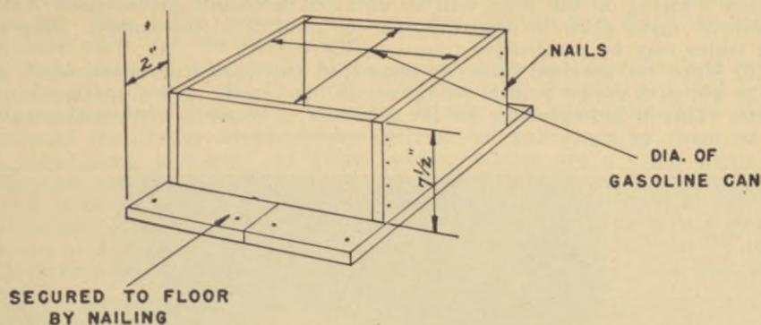
Plate 22. Container for gasoline can.
