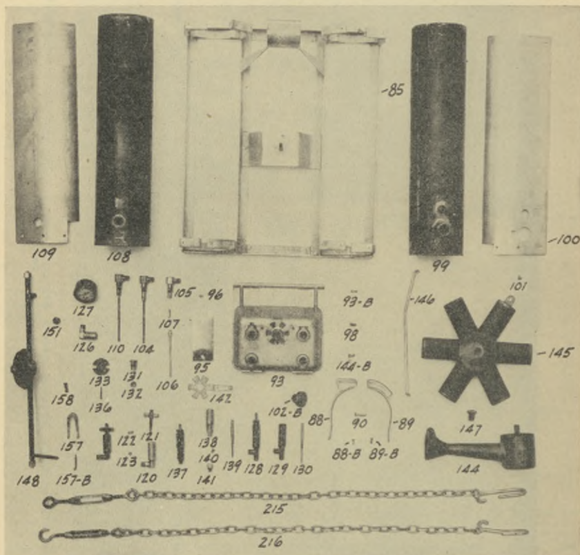
Plate 20. Fig. 1. Gasoline fire unit parts and tools.
