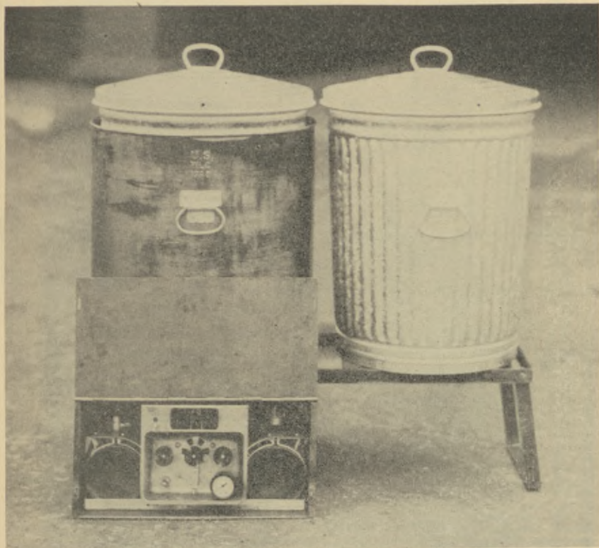
Plate 17. Water heater set up for use (case, can, can cover, and can shield).
