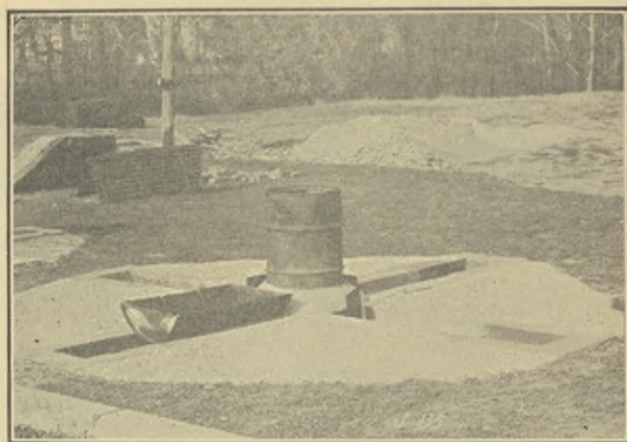
Plate 10. Cross Trench Incinerator made with 50-gallon Oil Drum. The Trenches are Longer than Normal in Order to Give Room for the Drying Pan.
