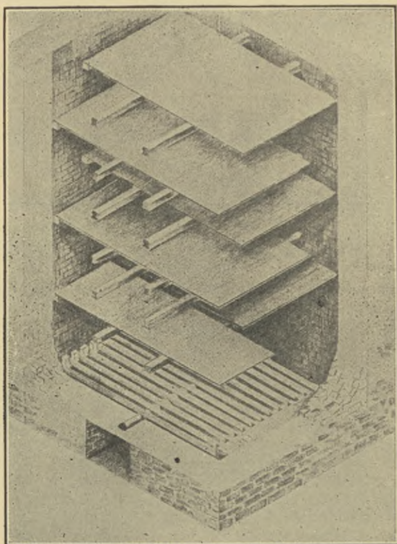
Plate 6. Multiple shed incinerator with side cut away to show interior construction
