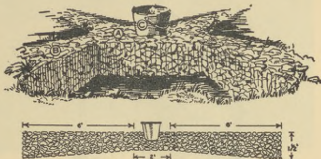
Plate 19. Soakage Trench.
