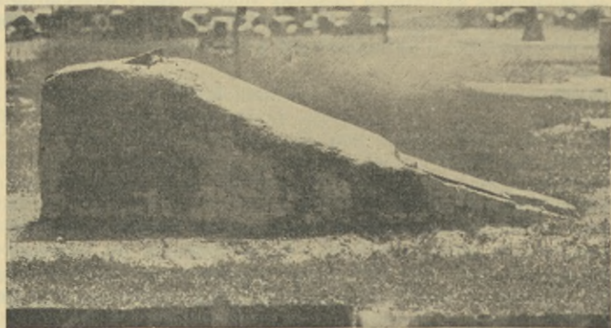
Plate 4. Incline Plane Incinerator, Side View.
