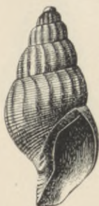
ALASKAN SPECIES OF CHRYSODOMUS. For explanation of plate see page 732.
