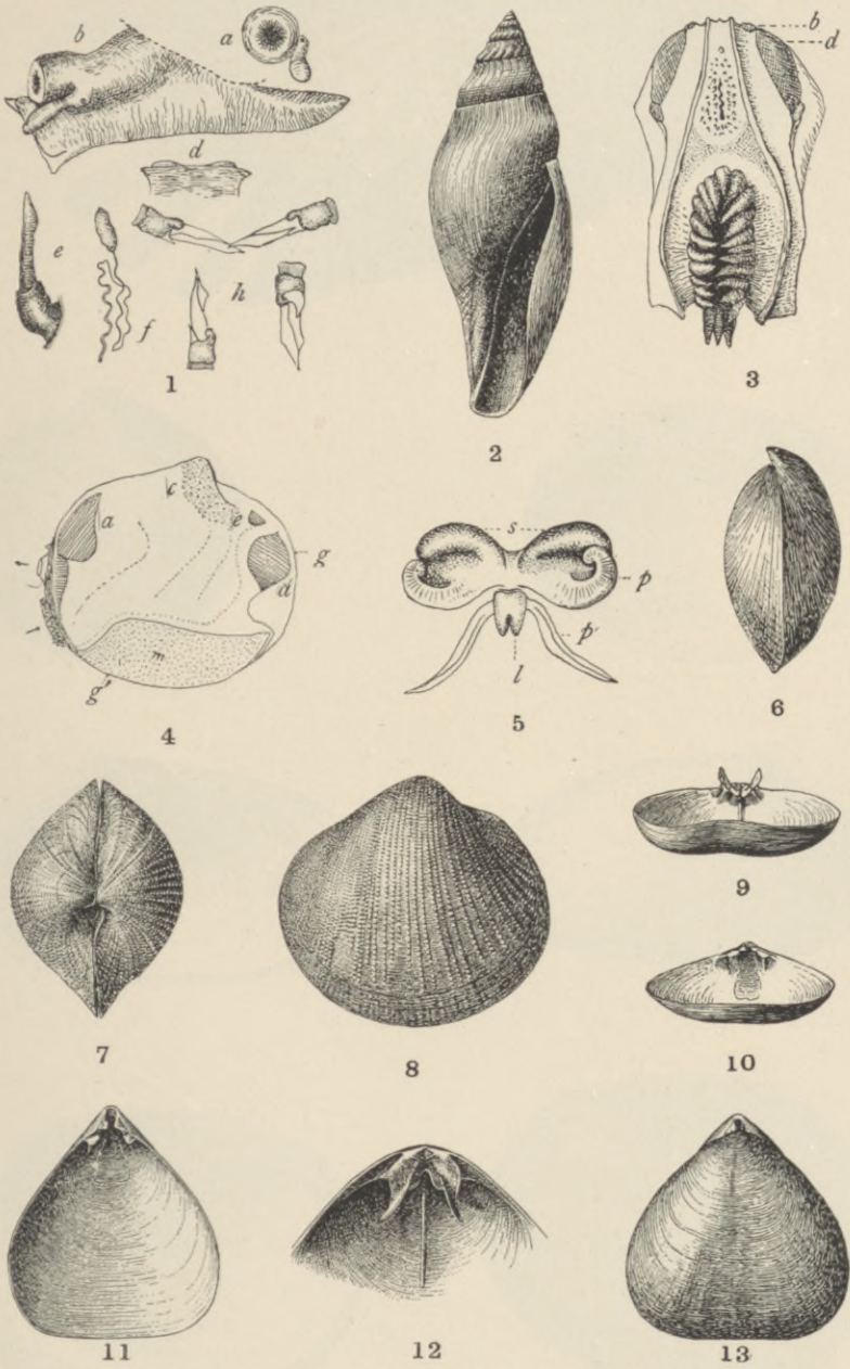
PACIFIC SHELLS AND BRACHIOPODS. For explanation of plate see page 731.
