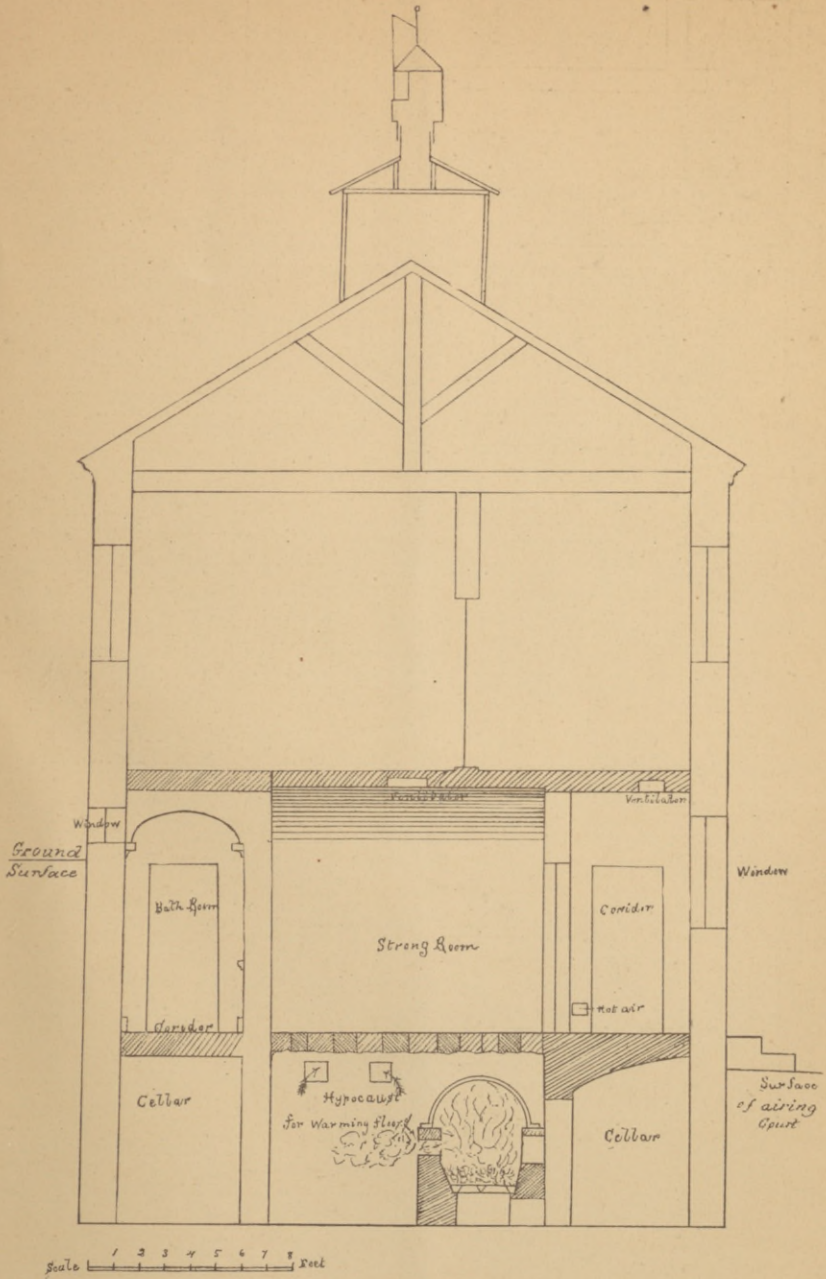
SECTION OF THE LODGE.
