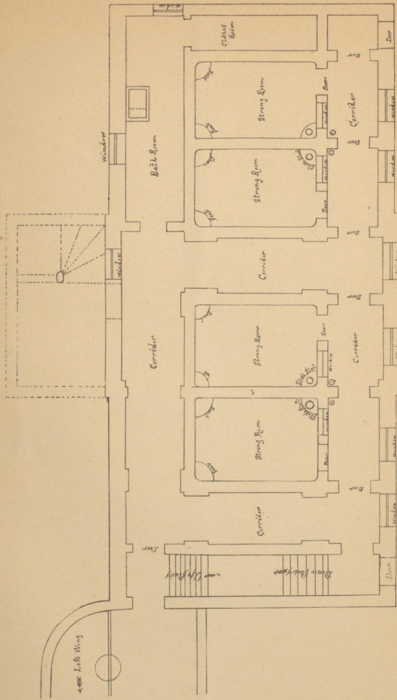
PLAN OF THE LODGE.
