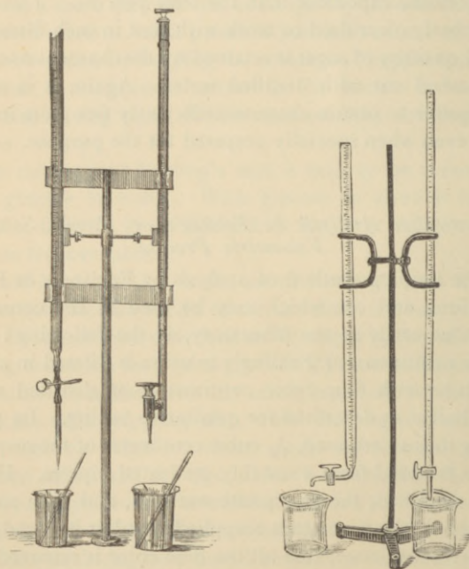
FIG. 7.—Varieties of Burette Stand.
