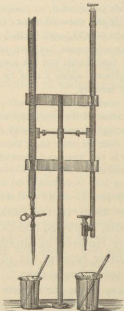
FIG. 14.—Burette Stand with Two Forms of Burette.
