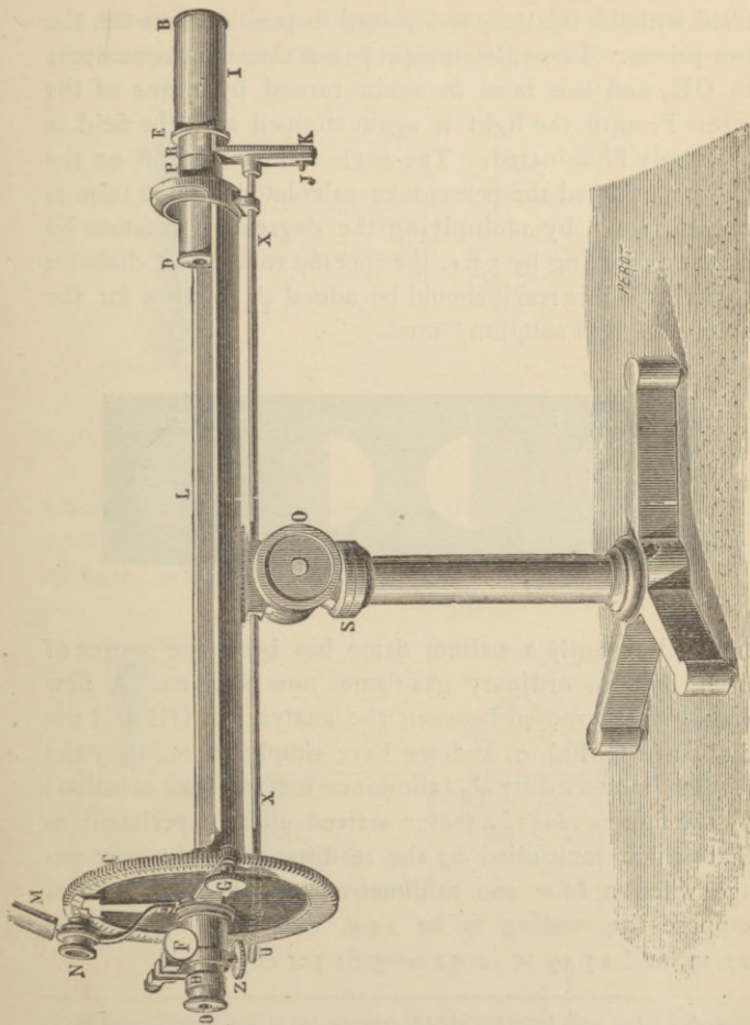
FIG. 9.—The Laurent Shadow Polarizing Saccharimeter.
