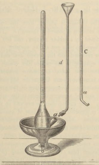
FIG. 15.—Marshall's Apparatus.
