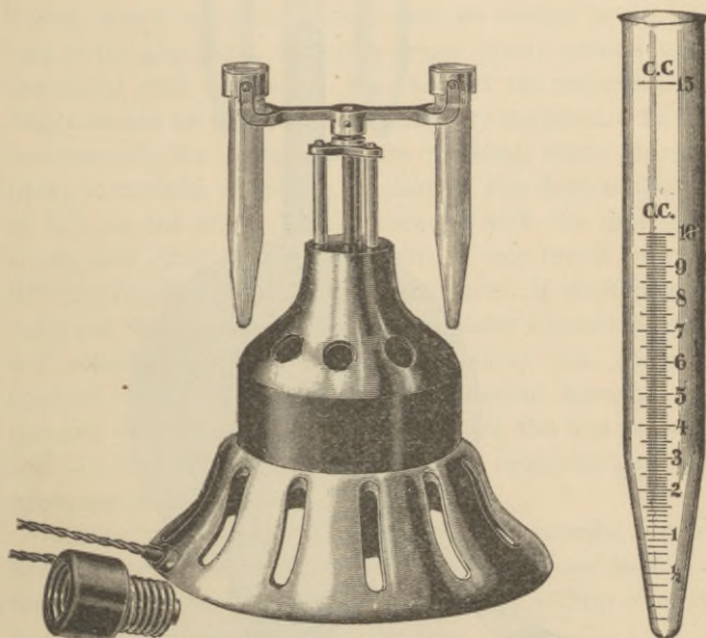
FIG. 44.—The Purdy Electric Centrifuge.
