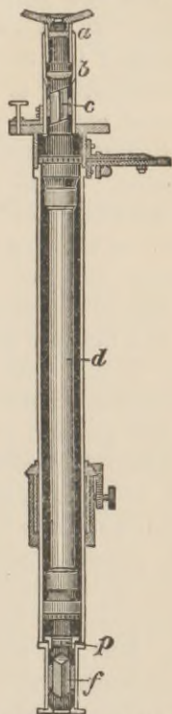
FIG. 11.—SECTIONAL VIEW OF ULTMANN'S POLARIZING SACCHARIMETER.
