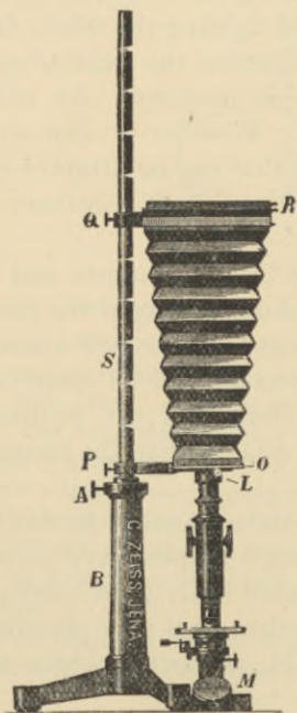
FIG. 158. Zeiss' Vertical Photo-micrographic Camera. A. Set screw holding the rod (S) in any desired position. P, Q. Set screws by which the bellows are held in place. B. Stand with tripod base in which the supporting rod (S) is held. This rod is now graduated in centimeters and is a ready means of determining the length of the camera. M. Mirror of the microscope. L. The sleeve serving to make a light tight connection between the camera and microscope. O. The lower end of the camera. R. The upper end of the camera where the focusing screen and plate holder are situated. (From Zeiss' Photo-micrographic Catalog).
