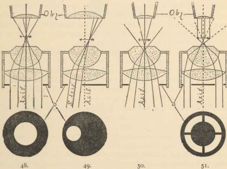
FIGS. 48-51. Sectional views of the Abbe Illuminator of 1.20 N. A. showing various methods of illumination (§ 84). Fig. 48, axial light with parallel rays. Fig. 49, oblique light. Fig. 50, axial light with converging beam. Fig. 51, dark-ground illumination with a central stop diaphragm.
