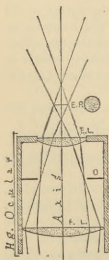
FIG. 30. Sectional view of a Huygenian ocular ( Hg. ocular ), to show the formation of the Eye-Point.
