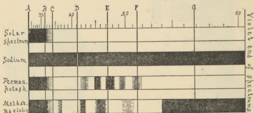
FIG. 115. Various Spectra. —All except that of Sodium were obtained by diffused day-light with the slit of such a width as gave the most distinct Fraunhofer lines.
