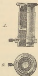
FIG. 139. Czapski's Ocular Iris-diaphragm with cross hairs for examining and accurately determining the axial images of small crystals. The iris diaphragm enables the observer to make the field as large or small as desired.
