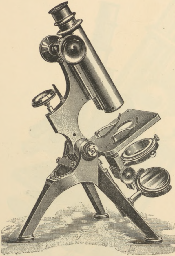
FIG. 71. Watson & Sons' Edinburgh Students' Microscope (Stand G). This is a good representative of the tripod-base, English models of to-day. It is in general like the Powell and Lealand stands which have held their position with the foremost English microscopists for the last 40 years. (See Carpenter-Dallinger, p. 172).
