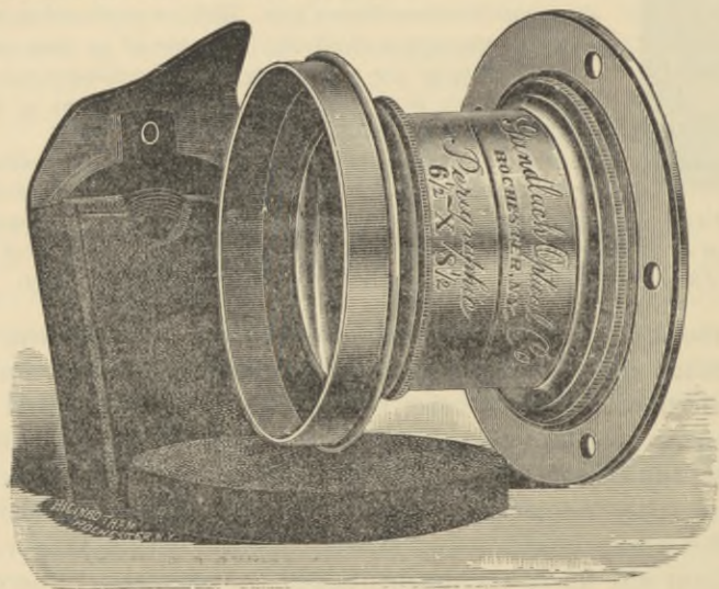
FIG. 151. Perigráfico Objective of about 90 millimeters equivalent focus for making photo-micrographs at a magnification of 2 to 15 diameters. It was found to give the best results when used right end to as in ordinary photography. (From the Gundlach Optical Co.)
