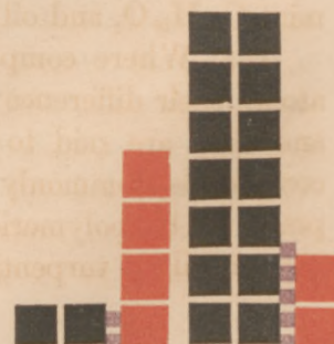
FORMOBENZOIC ACID.
