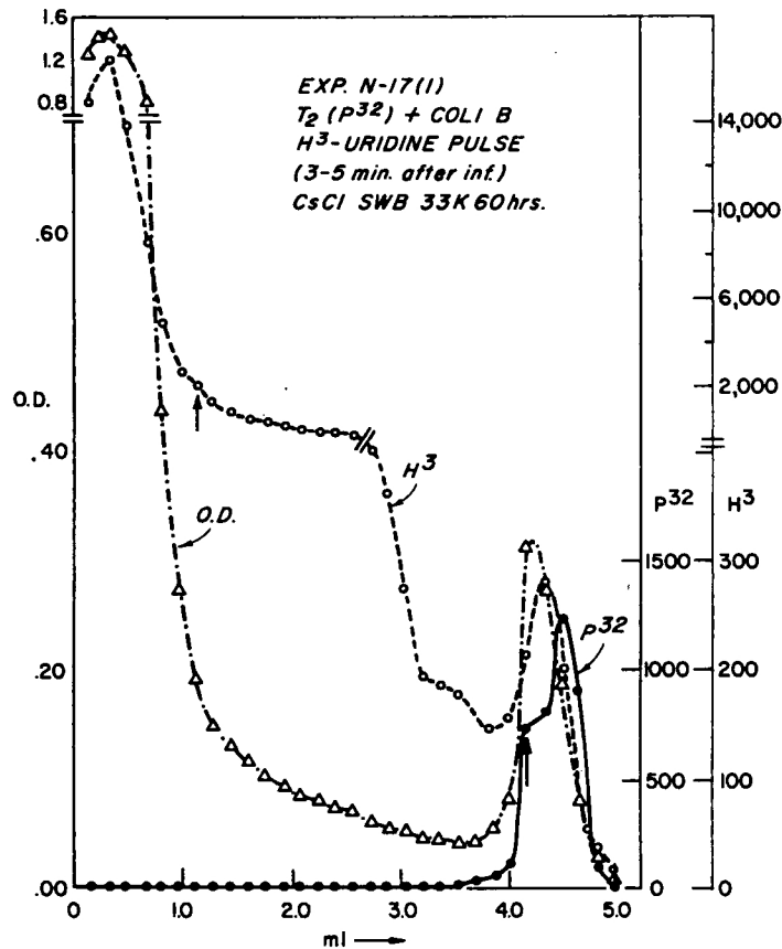
FIG. 2.—Adsorption of phage was carried out at a multiplicity of 15 of undiluted P^{32} -labeled virus. Pulsing was done between 3–5 minutes after 0 time with H^3 -uridine having a specific activity of 530 \mu\text{c}/\mu\text{M} at a level of 1 \mu\text{g}/\text{ml} . All other details are as described under Methods . Note that the radioactivity scale is expanded in the hybrid region.
