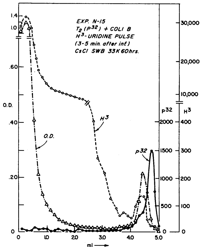
FIG. 1.—Adsorption of phage was carried out at a multiplicity of 45. P^{32} -labeled phage diluted 2-fold with unlabeled virus. Pulsing was done between 3–5 minutes after 0 time with H^3 -uridine having a specific activity of 1,600 \mu\text{c}/\mu\text{M} at a level of 0.3 \mu\text{g}/\text{ml} . All other details are as described under Methods . Note that the radioactivity scale is expanded in the hybrid region.
