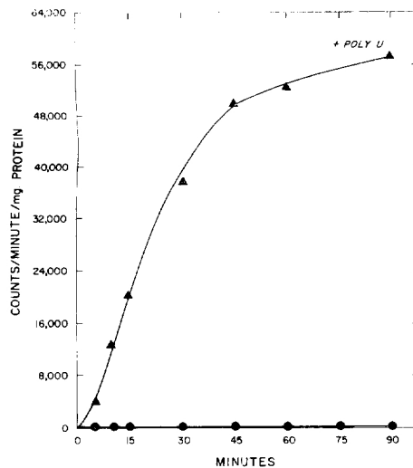
Fig. 6.—Stimulation of U- 14 C-L-phenylalanine incorporation by polyuridylic acid. ● without polyuridylic acid; ▲ 10 µg polyuridylic acid added. The components of the reaction mixtures and the incubation conditions are given in Table 1. 0.024 µmole U- 14 C-L-phenylalanine (~500,000 counts/min) and 2.3 mg Incubated-S-30 protein were added/ml of reaction mixture.
