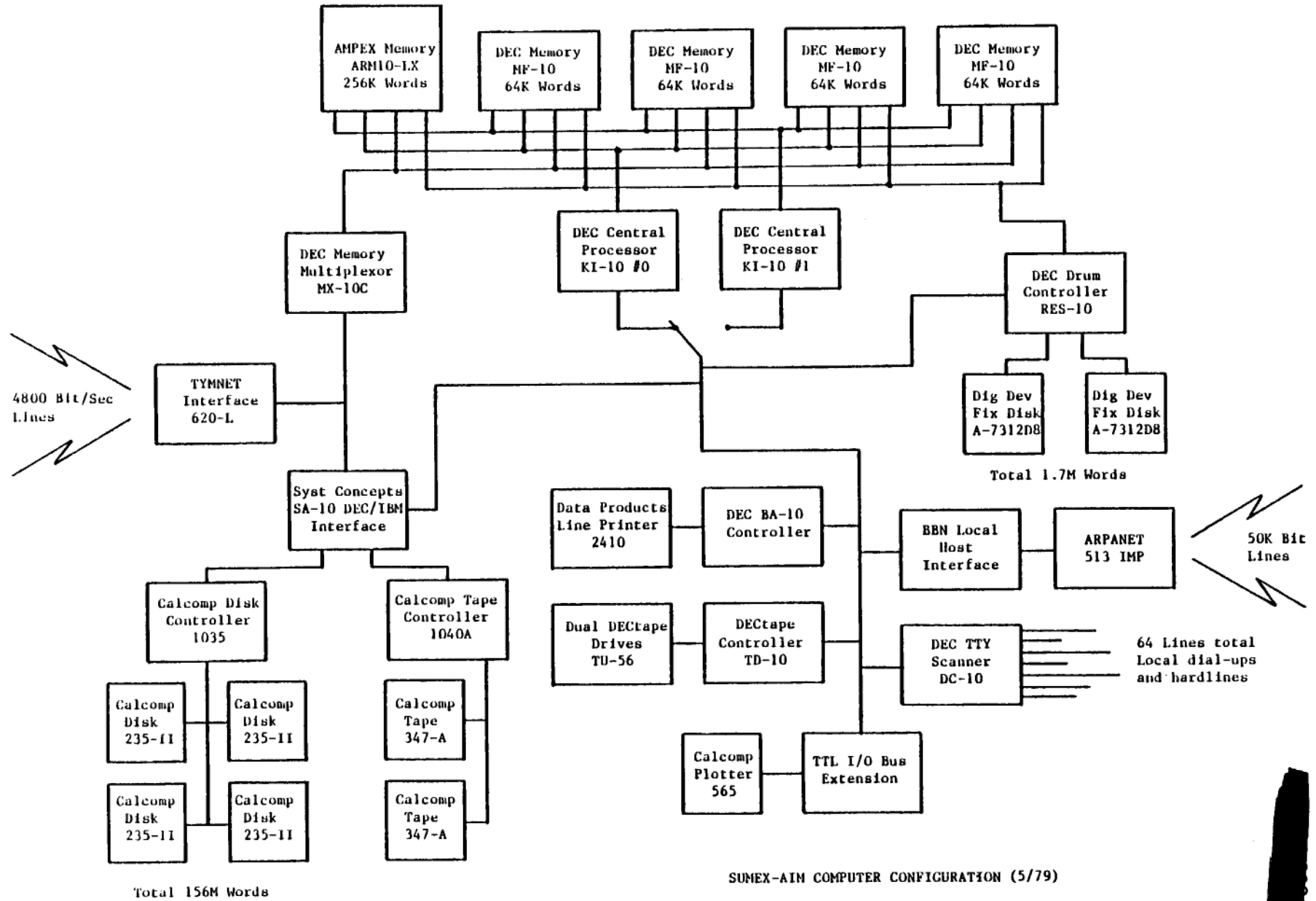
Figure 11. SUMEX hardware
