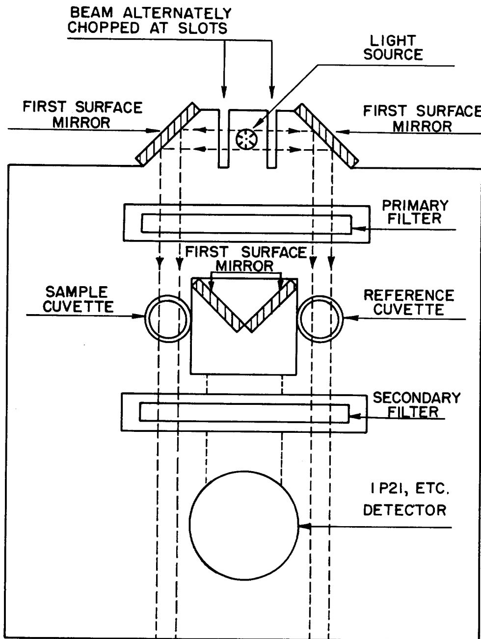
Figure 6. Fluorometry Test Unit Mark III
