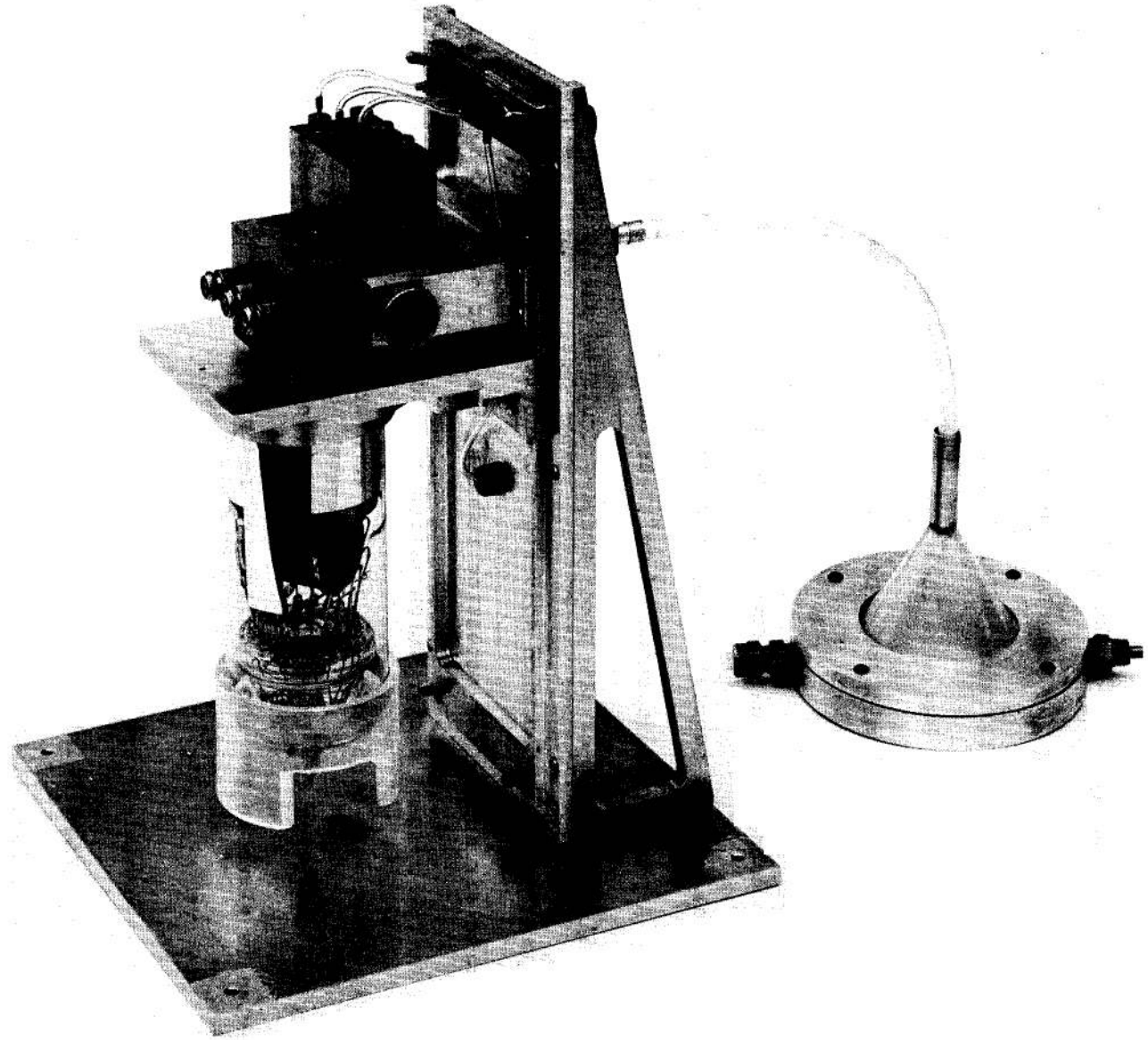
Figure 1. Field-Test Multivibrator
