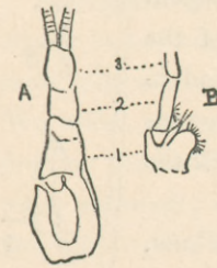
FIG. 18. Inner antennæ. A., of lobster; B., of Palaemon .
