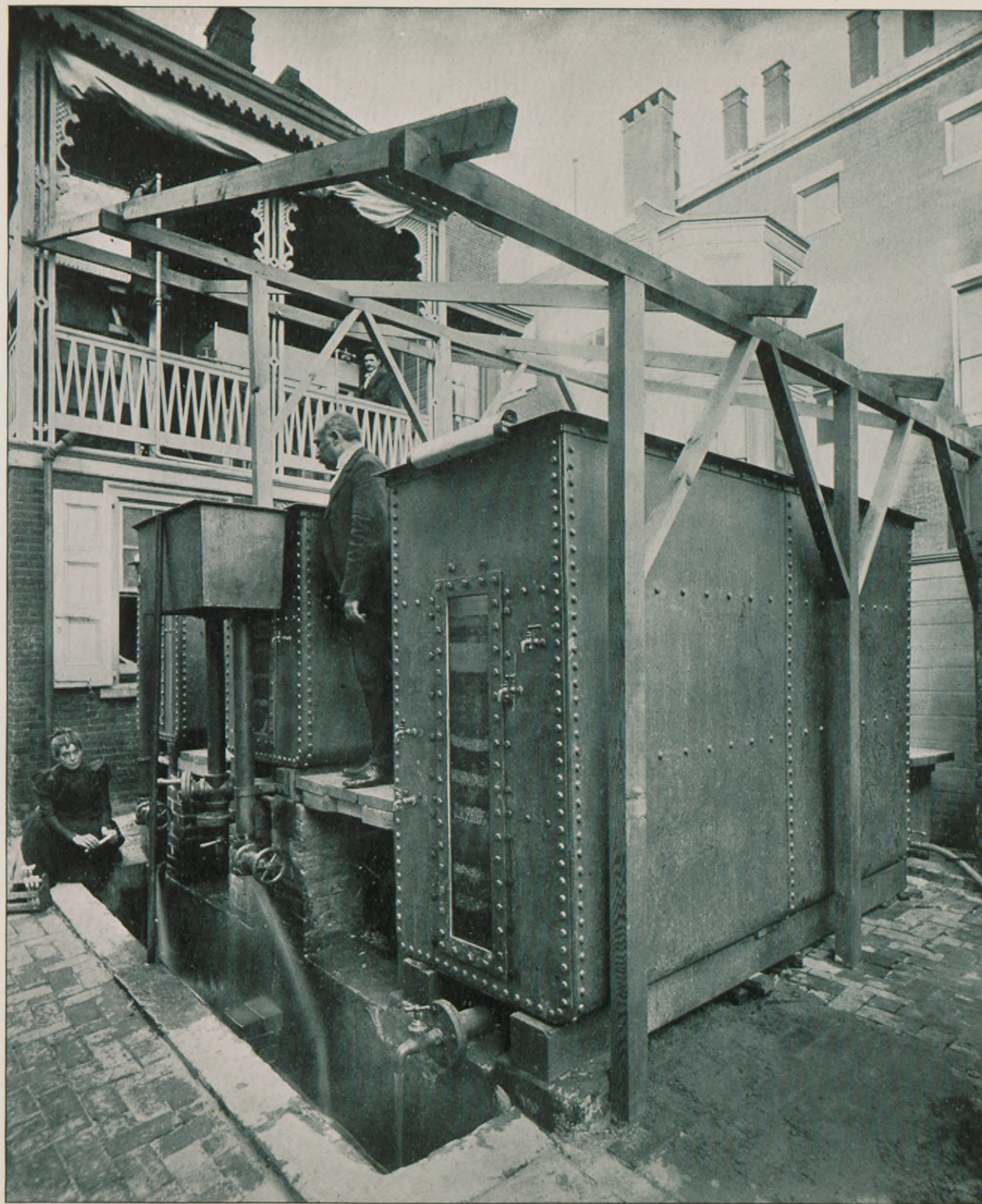
Figure 5. Maignen's Improved Sand Filtration Experimental Plant. 1310 Arch St., Philadelphia.
