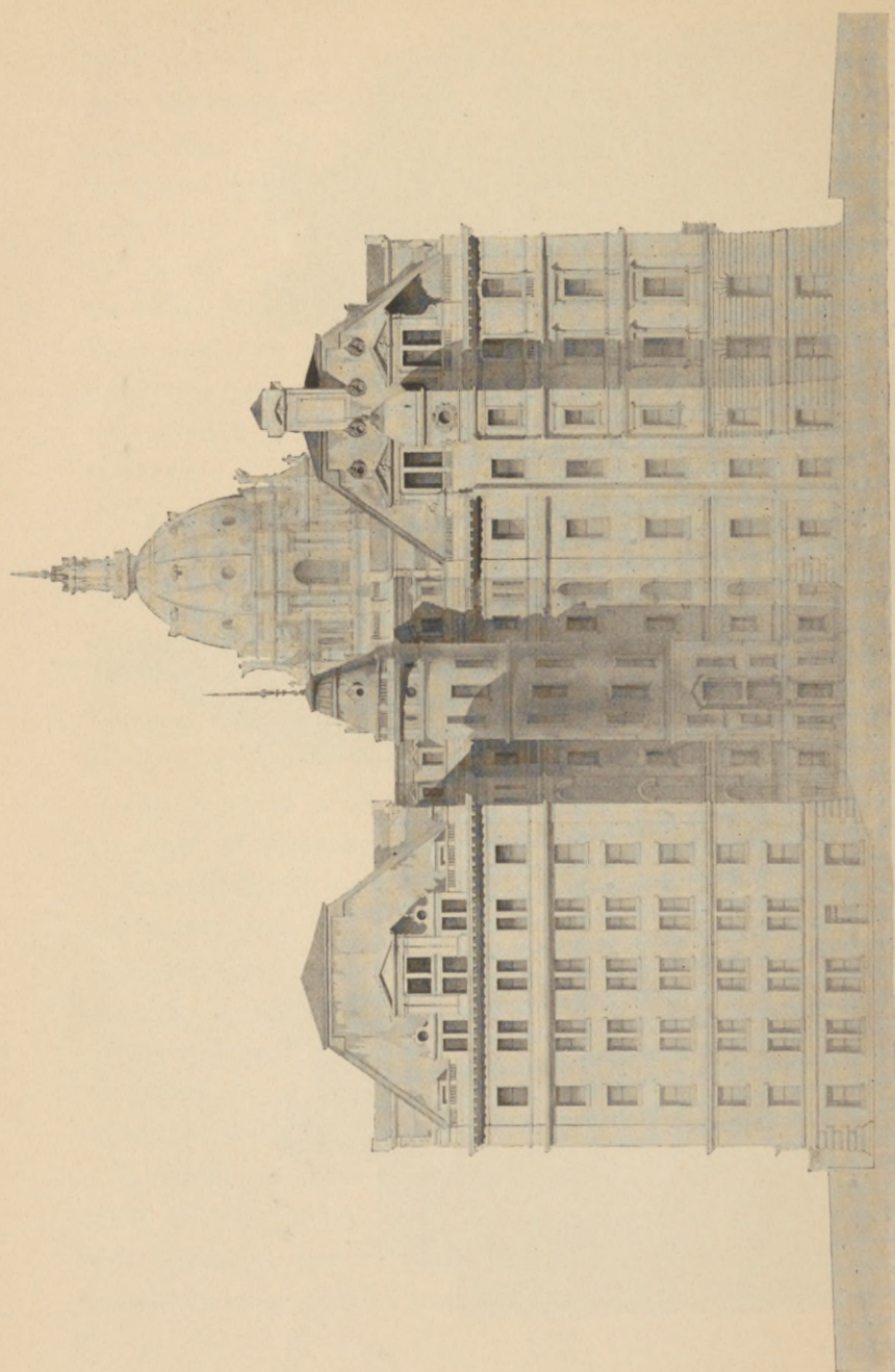
WESTERN ELEVATION: MUHLENBERG PAVILION IN CENTRE NORRIE PAVILION TO THE RIGHT, VANDERBILT PAVILION TO THE LEFT.
