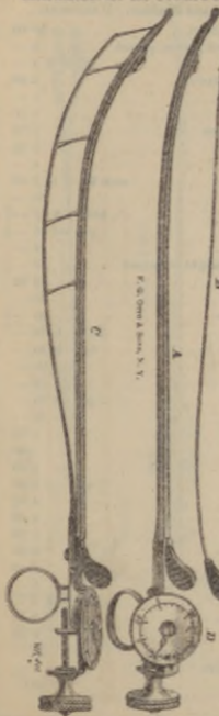
Olivé's Dilating Instrument Urethrotome Curved, No. 2.
