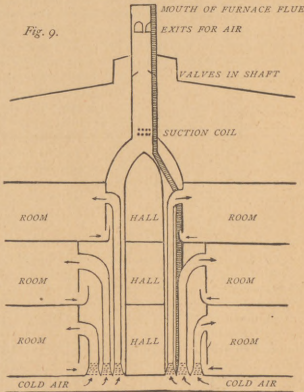
BRIDGEPORT, CONN., HIGH SCHOOL. Vertical Section.
