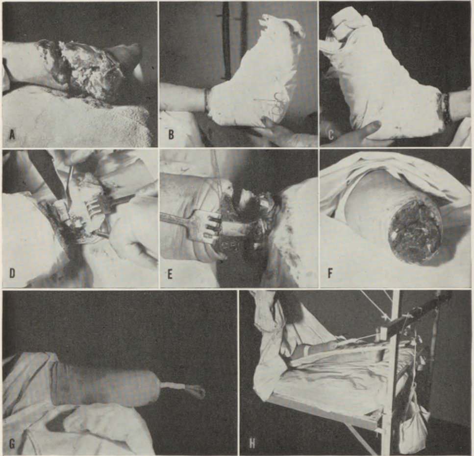
FIGURE 86.—Technique of open circular amputation. A. Severe injury in region of right ankle, with established infection, for which secondary amputation was performed in a fixed hospital. Note destruction of heel. B. Lateral view of circular incision through skin, which has retracted. C. Medial view of incision of fascia and muscles at level to which skin has retracted in view B. D. Incision of periosteum, sawing of tibia, at level to which muscles have retracted in view C. E. Lateral view of section of fibula with Gigli saw at level slightly proximal to stump of tibia. In the open circular technique, no particular effort is made to section the fibula \frac{3}{4} to 1 inch above the end of the tibia, as is done at definitive reamputation or revision of the stump. F. Open concave circular stump at completion of amputation. G. Stockinet applied in fixed hospital after dressing of open circular stump. H. Skin traction provided by means of weight attached to rope which passes over pulley and extends from stockinet attached to skin; lower extremity rests on half-ring leg splint. This is the most effective means of traction on the skin following open circular amputation.
