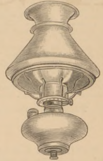
No. 4. FOUNT. plain and flat. B.X.L. Burner, 7 in. shade
