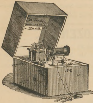
No. 2 Electro Magnetic Machine } 16 Cell Galvanic Battery. For Family Use. } (continuous current.) Highest Award received from Centennial Exposition, 1876.
