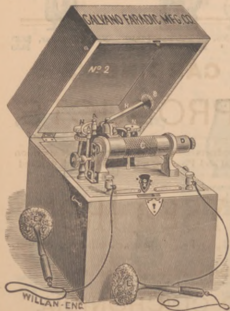
No. 2 Electro Magnetic Machine } For Family Use.
