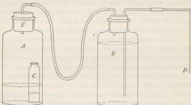
Apparatus for Determining Urea in Urine.
