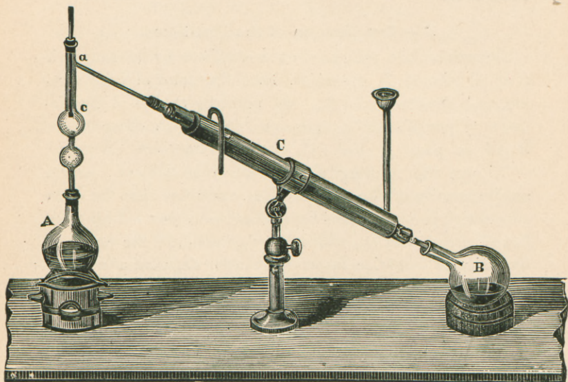
Fig. 6 shows the disposition of apparatus at the commencement of the distillation; so soon as the lighter products have passed over, the bulb tube ac must be removed and connection made with the condenser by a short bent tube.
