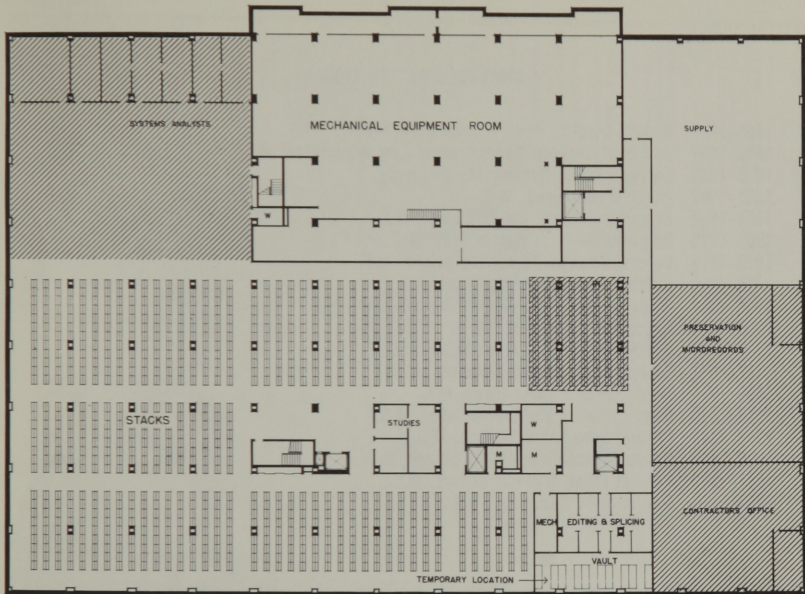
1967 FLOOR PLAN C LEVEL
