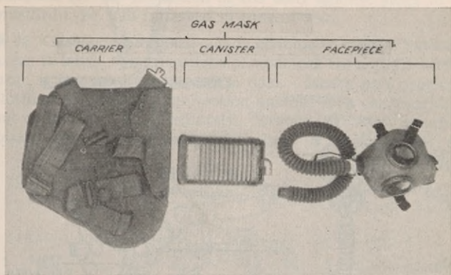
FIGURE 6.—Principal parts of service gas mask.
