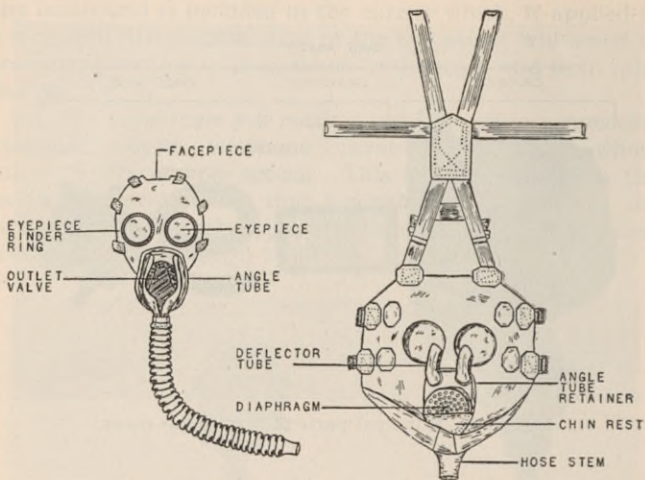
FIGURE 8.—Facepiece assembly, diaphragm.
