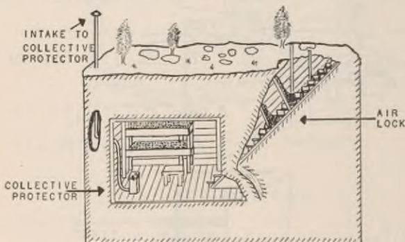
FIGURE 11.—Model of ideal dugout.
