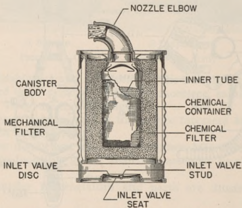
FIGURE 9.—Canister (sectionalized).
