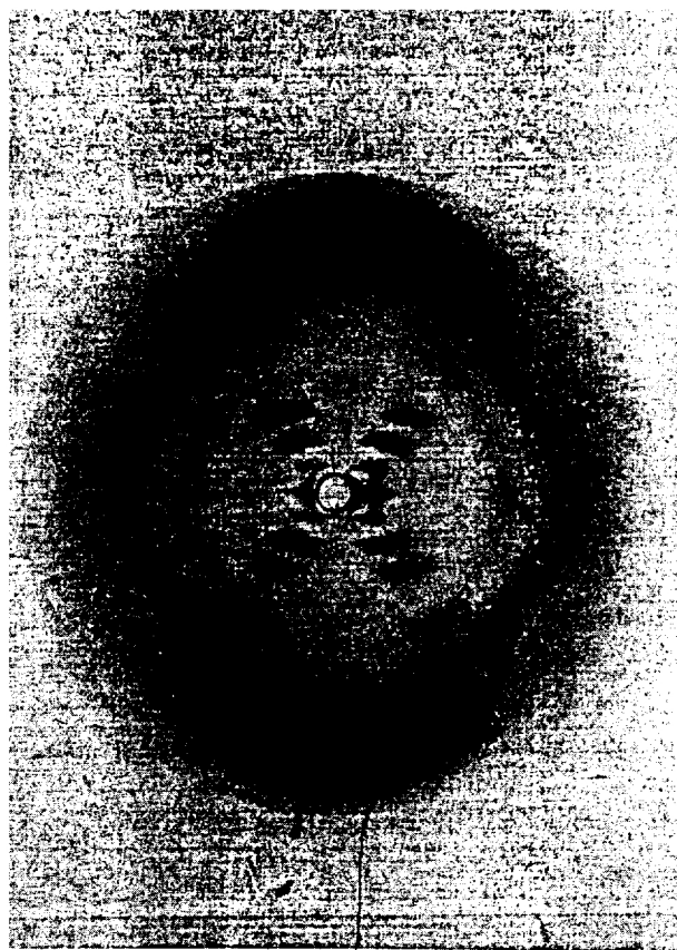
FIGURE 3. X-ray fiber diagram of Structure B of desoxyribonucleic acid. (R. E. Franklin and R. Gosling, 1953a.)
